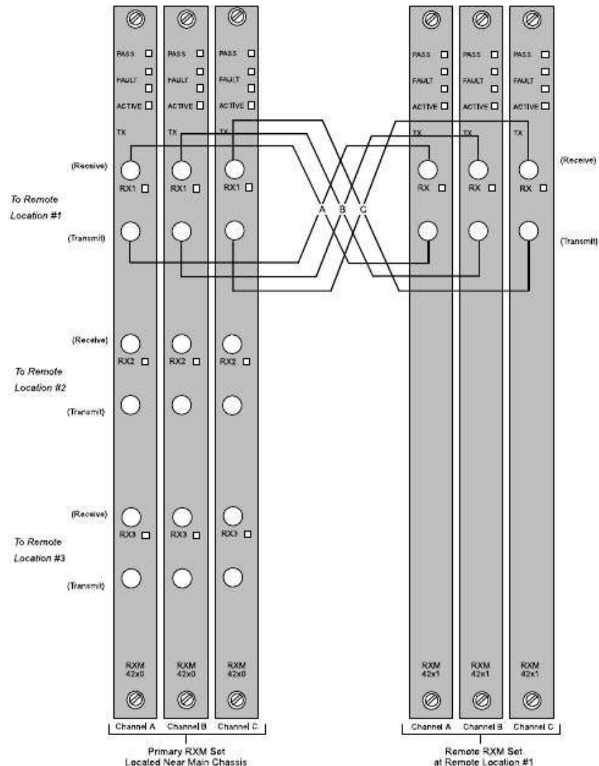
Sample Wiring for One Remote Location
